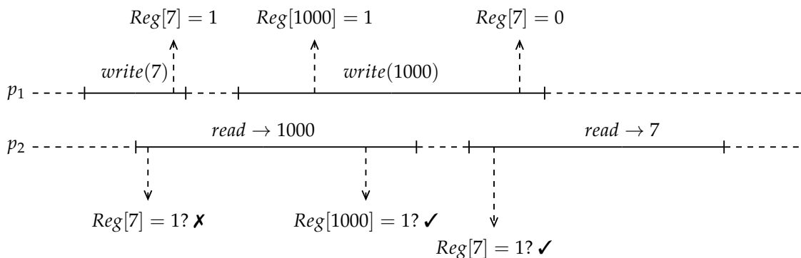
Figure 2: Execution that violates atomicity.
