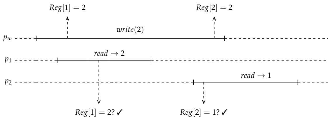
Figure 3: Execution that violates atomicity.
